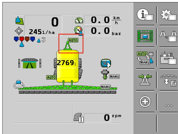
Abb. 68. TrailControl
