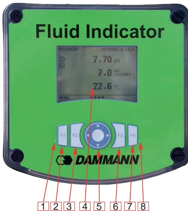
Abb. 88. Fluid Indicator
