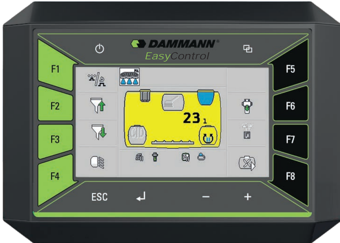
Abb. 80. EasyControl
