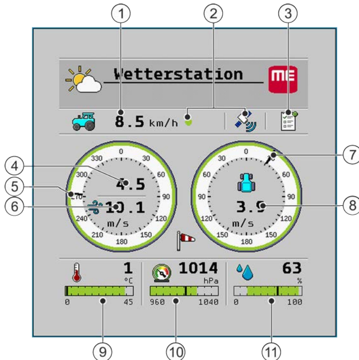
Abb. 104. Wetterstation
