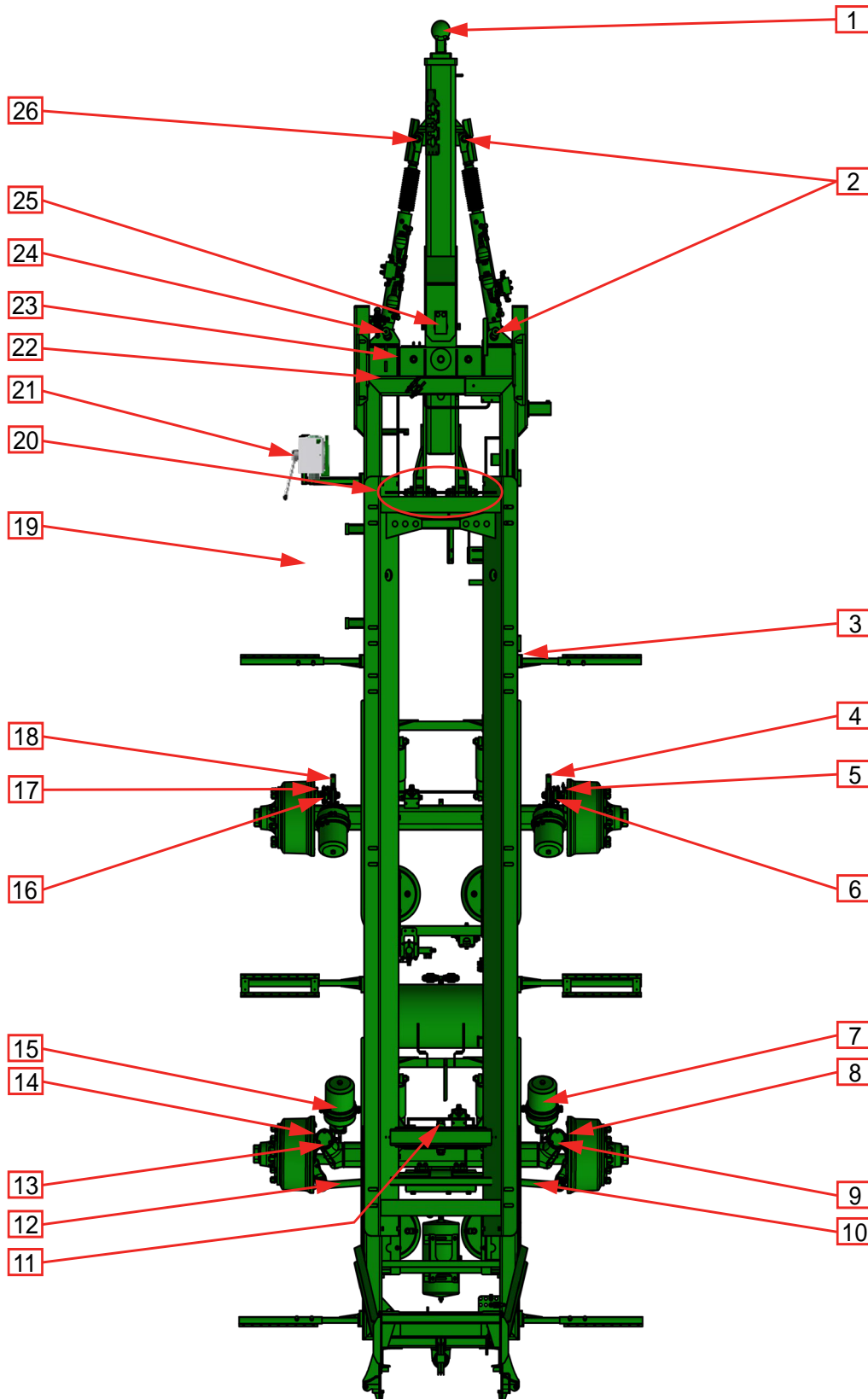
Abb. 115. Schmierplan Profi-Class Tandem
